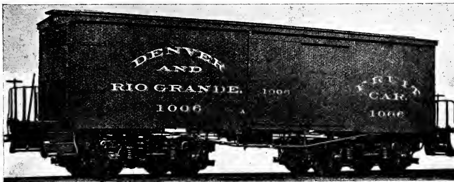
Fig. 6. FRUIT CAR. DENVER & RIO GRANDE RAILROAD. Length, 34 ft. Capacity, 40,000 lbs. Weight, 43,600 lbs. Equipped with Platforms and Steps, Passenger Trucks, End Ventilators and Air Brakes.
